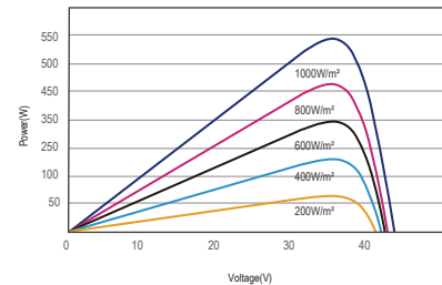
P-V Curves(550W)
