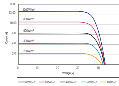
I-V Curves(550W)
